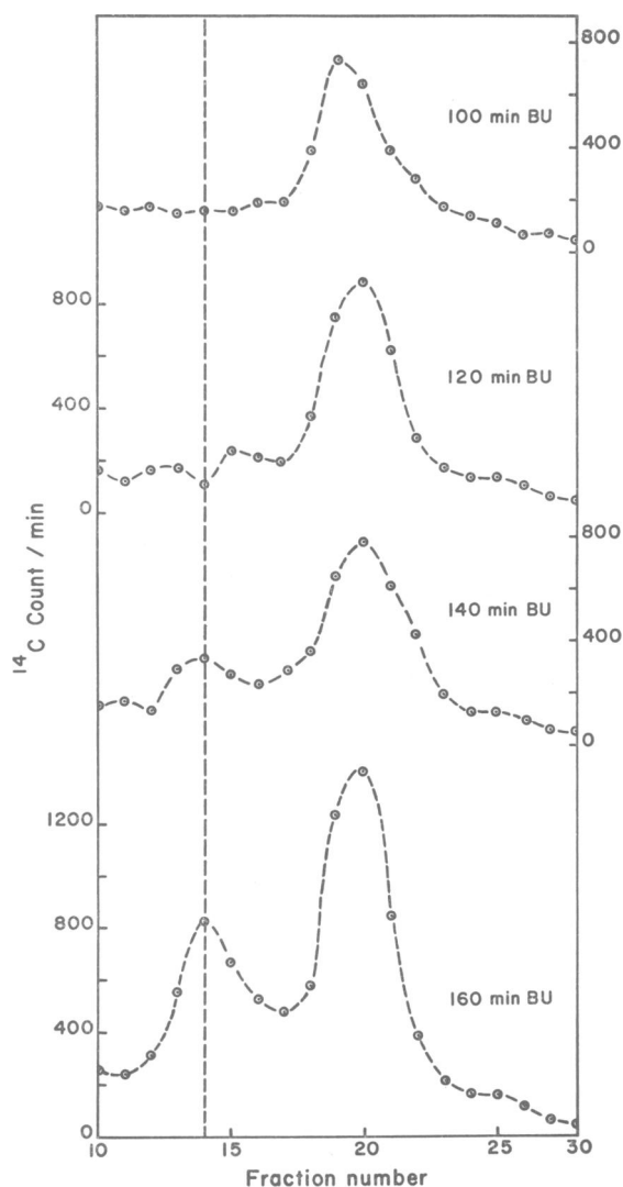
FIGURE 1 Radioactivity profile of density gradient sedimentation patterns of lysates of cells growing in glucose minimal medium. Bromouracil-5- 14 C was substituted for thymidine at 0.1 \mu C/ml for 100, 120, 140, and 160 min as indicated. The vertical line indicates the approximate position of DNA containing 5-bromouracil in place of thymine in both strands.
