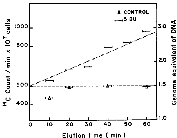
FIGURE 3 Incorporation of thymidine- ^{14}\text{C} into cells eluted from membrane-bound cultures. 100-ml cultures containing 1.0 \times 10^8 cells/ml growing in glucose minimal medium were bound to membranes, washed, and eluted at a rate of 3 ml/min with medium containing 4 \mu\text{g}/\text{ml} of 5-bromouracil. 4 min samples were collected at 10, 20, 30, 40, 50, and 60 min after the start of elution and were poured into culture flasks containing 1 \mu\text{C} of thymidine- ^{14}\text{C} and 40 \mu\text{g} of unlabeled thymidine. After 40 min of incubation at 37^\circ\text{C} with shaking, the incorporation of the radioactive label was stopped by adding cold trichloroacetic acid and excess unlabeled thymidine. Control cultures were eluted with 4 \mu\text{g}/\text{ml} thymidine and treated in a similar way. The bar indicates the length of the collection time. The straight lines (dotted, C = 120 ; dashed, C = 40 ) represent the potential for DNA replication calculated assuming the accumulation of initiator. The C = 120 min line was determined by calculating (1) the time of division of individual cells in an exponentially growing culture after the shift from C = 40 to C = 120 , (2) the chromosome configurations and the amount of initiator at division, and (3) the number of genome equivalents of DNA replicated in a 40 min period following restoration of C = 40 min. The C = 40 min curve was determined by calculating the number of genome equivalents replicated in a 40 min period by newborn cells with C = 40 min.
